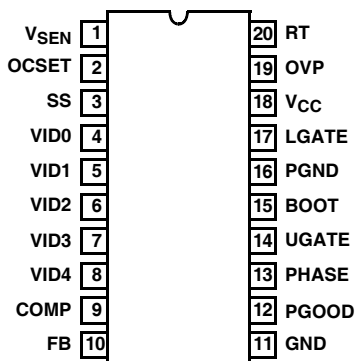
HIP6014 (SOIC) TOP VIEW
